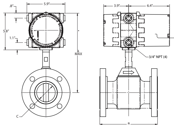
Figure 6. Dimensions: Flange Connection, Integral Mounting.
