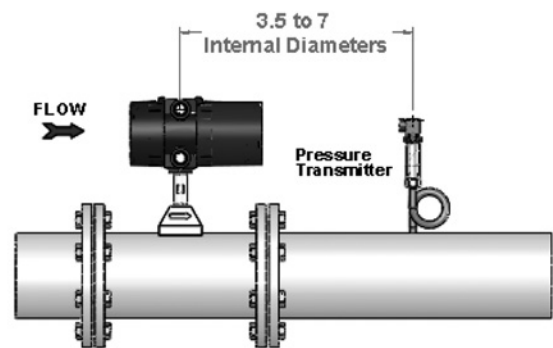
Figure 3. Pressure Tap Dimensions.
