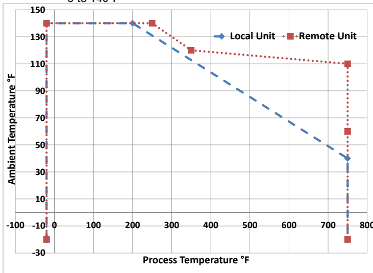
Figure 1. Ambient Temperature Range for Integral and Remote Mounted Electronics
