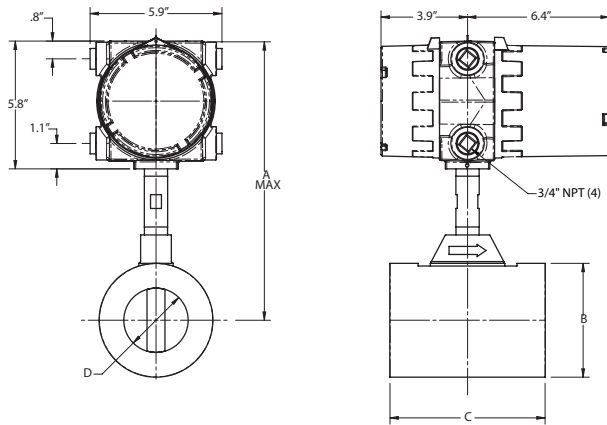
Figure 4. Dimensions: Wafer Connection Type, Integral Mounting.
