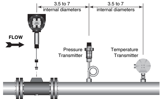
Figure 3. Pressure and Temperature Tap Dimensions.
